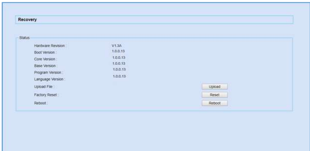
Figure 351: Recovery Mode
