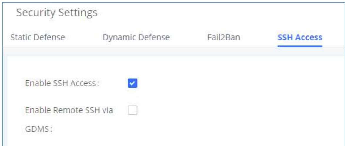
Figure 34: SSH Access
