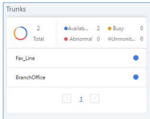
Figure 284: Trunk Status
