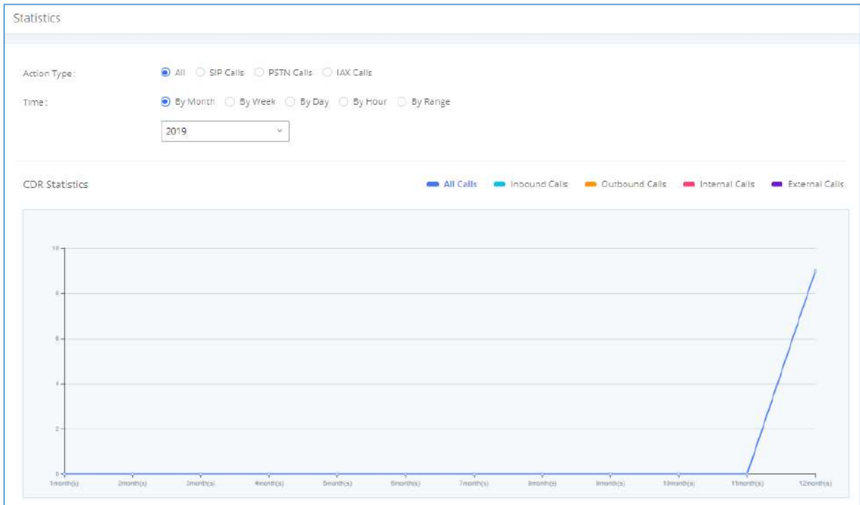
Figure 310: CDR Statistics
