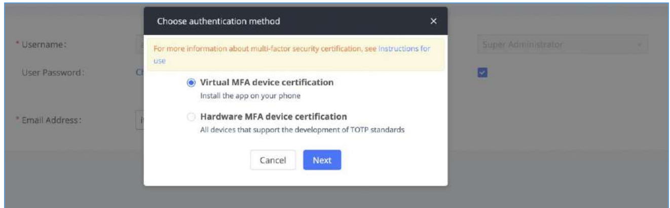
Figure 318: MFA Settings
