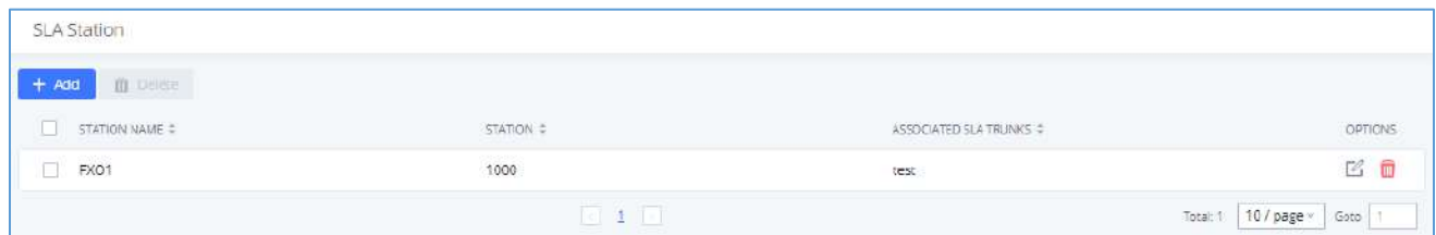
Figure 108: SLA Station
